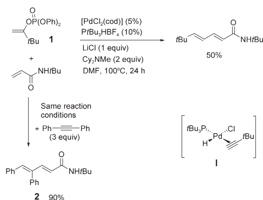
Scheme 1. Crossover experiment with diphenylacetylene. cod = 1,5-cyclooctadiene, Cy = cyclohexyl, DMF = N,N -dimethylformamide.
