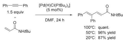
Scheme 4. Intermolecular ene-yne coupling catalyzed by [Pd(H)Cl-( Pt Bu 3 ) 2 ].
