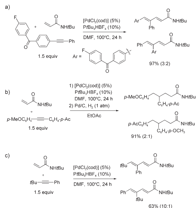
Scheme 2. Intermolecular ene-yne coupling with disubstituted non-symmetrical acetylenes.
