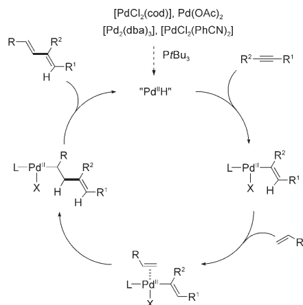
Scheme 3. Proposed mechanism of the intermolecular ene-yne coupling. dba = dibenzylideneacetone.
